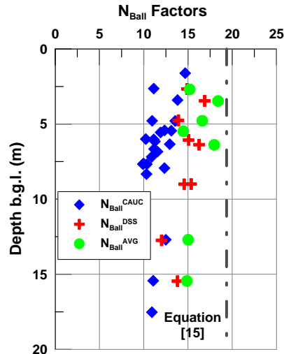
Figure 2. N_{Ball} against depth varying with shear strength source (Boylan et al, 2007)
