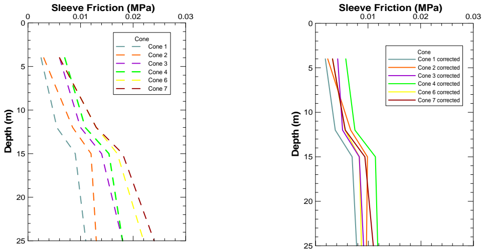
Figure 3. Uncorrected and Corrected f_s profiles for different cones at Onsoy
