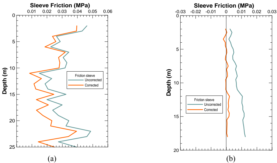
Figure 4. (a) Correction and (b) Over correction of Sleeve Friction
