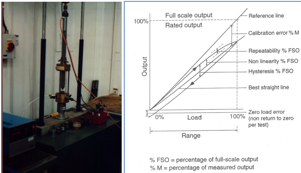
Figure 5. a) Calibration arrangement for CPTU and b) Calibration features for electronic transducers (after Lunne et al. 1997).
