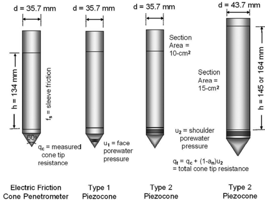
Figure 1. Standard dimensions of piezocones (Mayne 2007).
