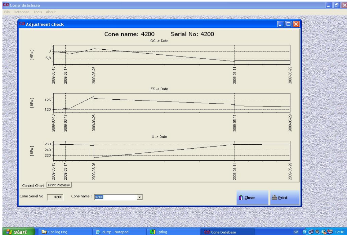
Figure 6. History of zero load readings for a Geotech piezocone ( www.geotech.se ).
