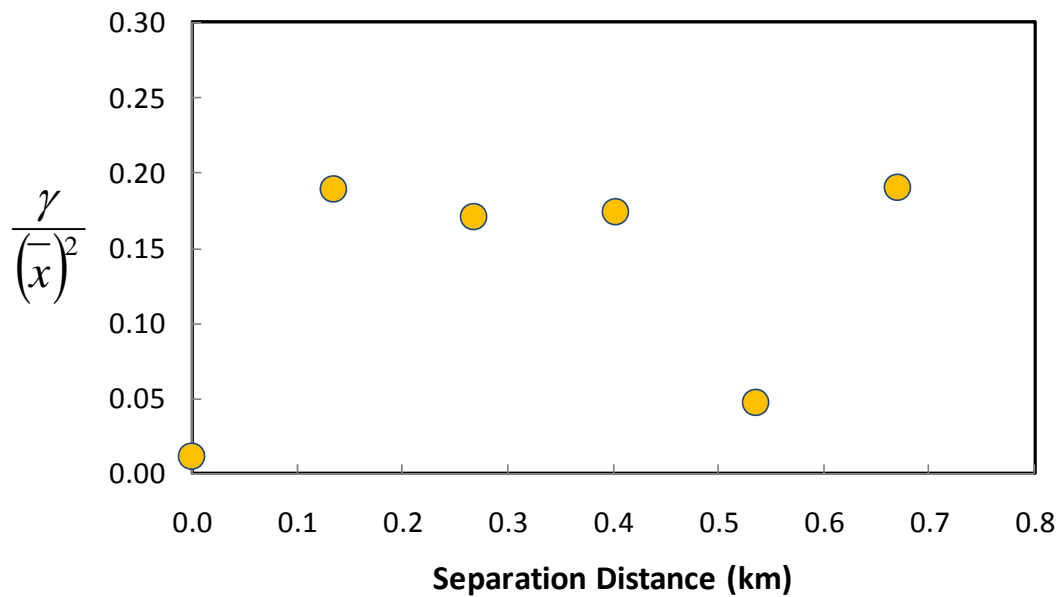
Figure 5. General relative variogram of the peaty organic foundation material. The plateau at a shorter separation distance is consistent with the smaller scale depositional environment of peaty organic materials.
