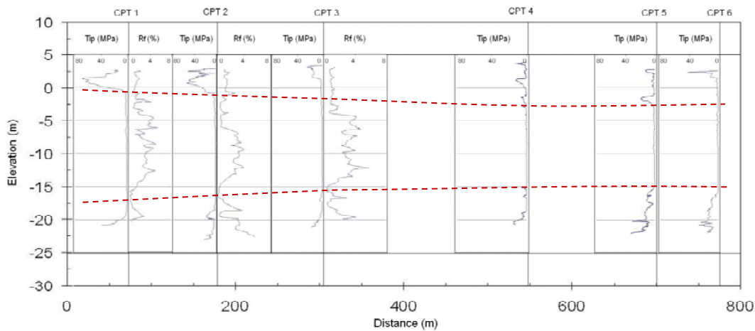
Figure 2. Six levee crest CPT soundings spatially located with respect to each other. Shown are the sounding and an interpretation of soil stratigraphy.
