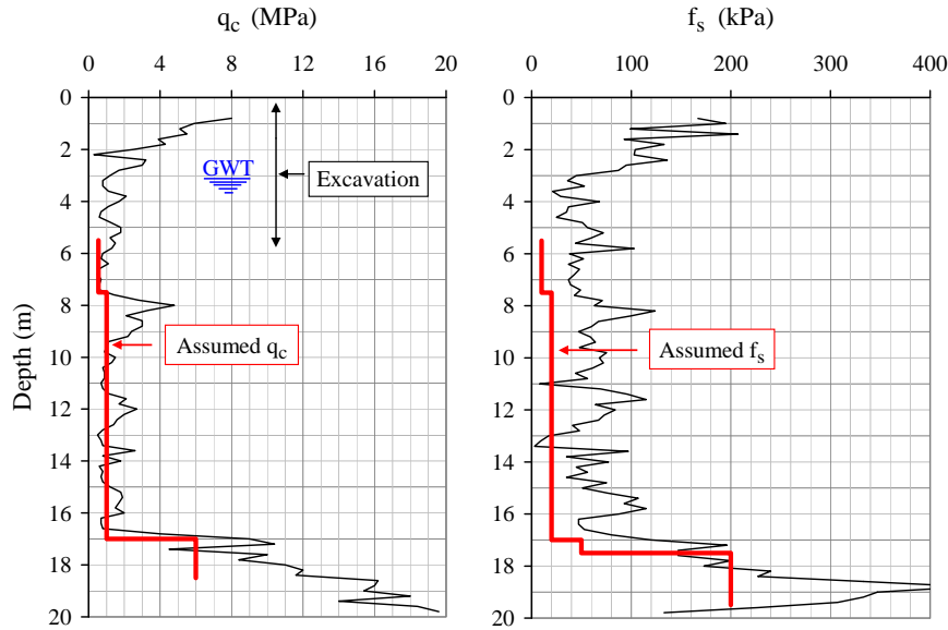
Figure 1. CPT2 Histograms
