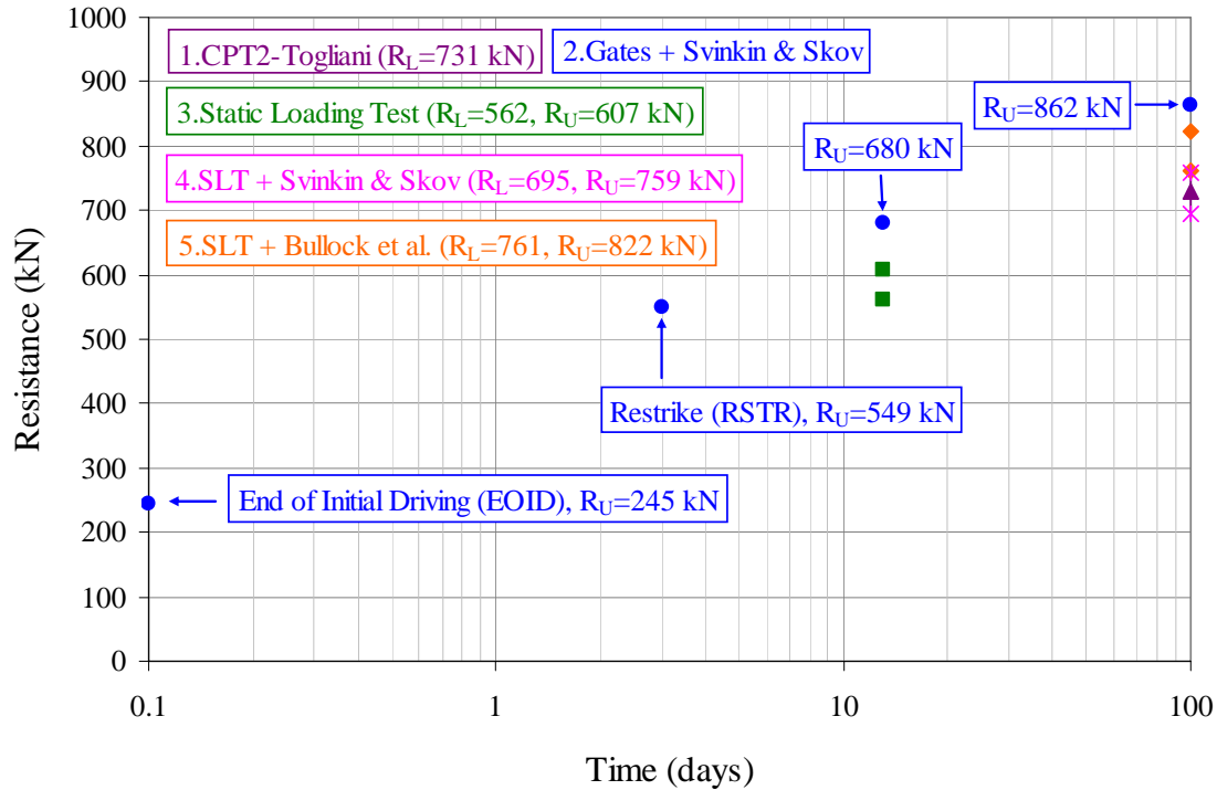
Figure 6. Pile Capacities
