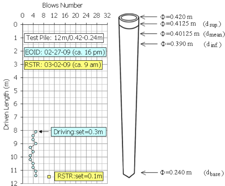
Figure 2. Penetration Log and Pile Sketch
