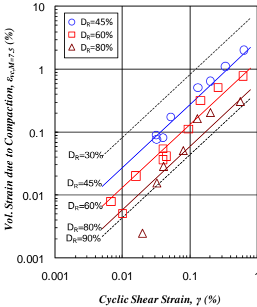
Figure 5. Relationship between volumetric strain and shear strain for dry clean sands (after Silver & Seed 1971)
