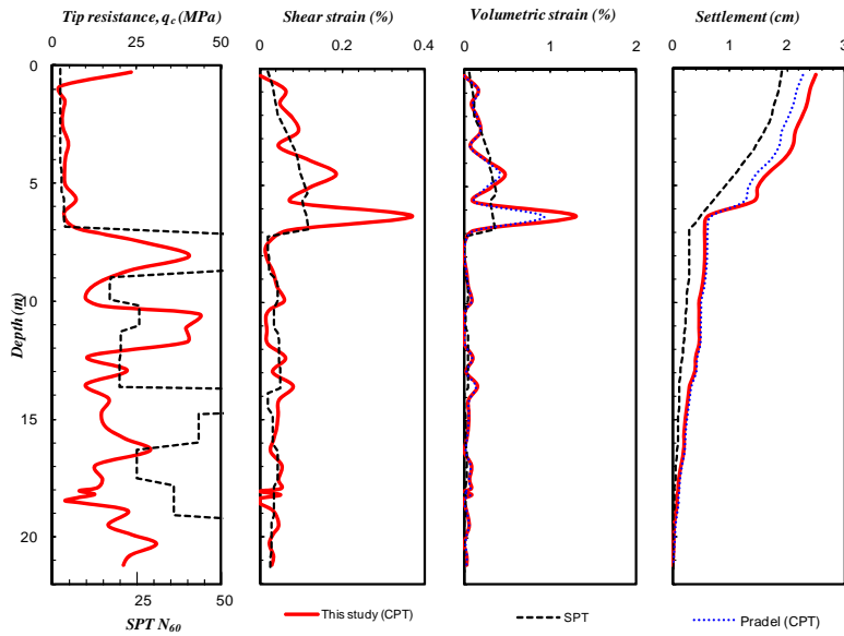
Figure 7. Calculated shear strain, volumetric strain, and settlement of dry sand for Site A
