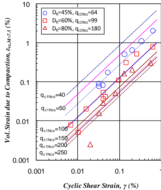
Figure 6. Relationship between volumetric strain, shear strain and normalized CPT tip resistance for dry clean sands
