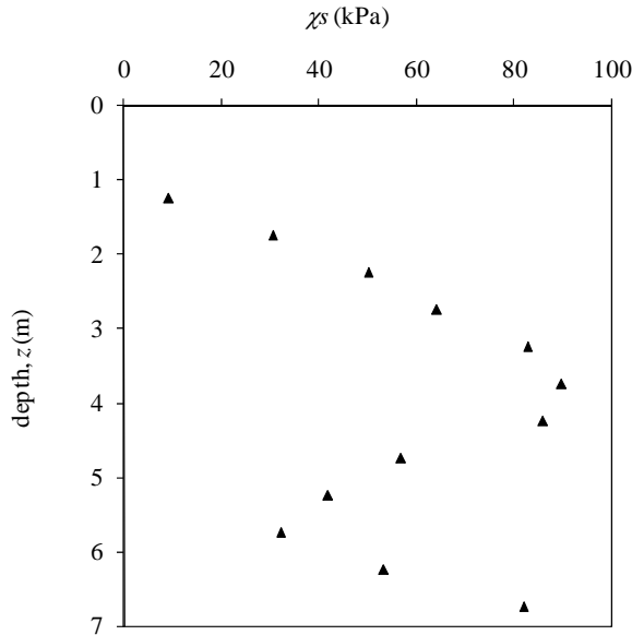
Figure 3. \chi_s back-calculated from cone penetration resistance using Equation 9.
