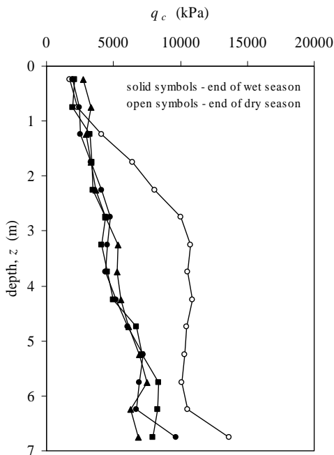
Figure 2. Cone penetration resistance for Perth sand in a treed area at the ends of wet and dry seasons (after Lehane et al., 2004).
