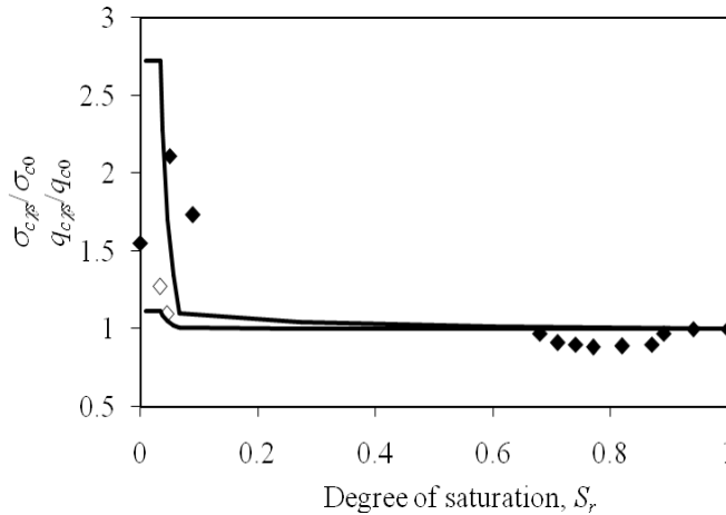
Figure 1. Normalized cone penetration resistances (symbols) and cavity expansion pressures (continuous lines) plotted against degree of saturation, for mean net stresses of 5 kPa and 100 kPa.
