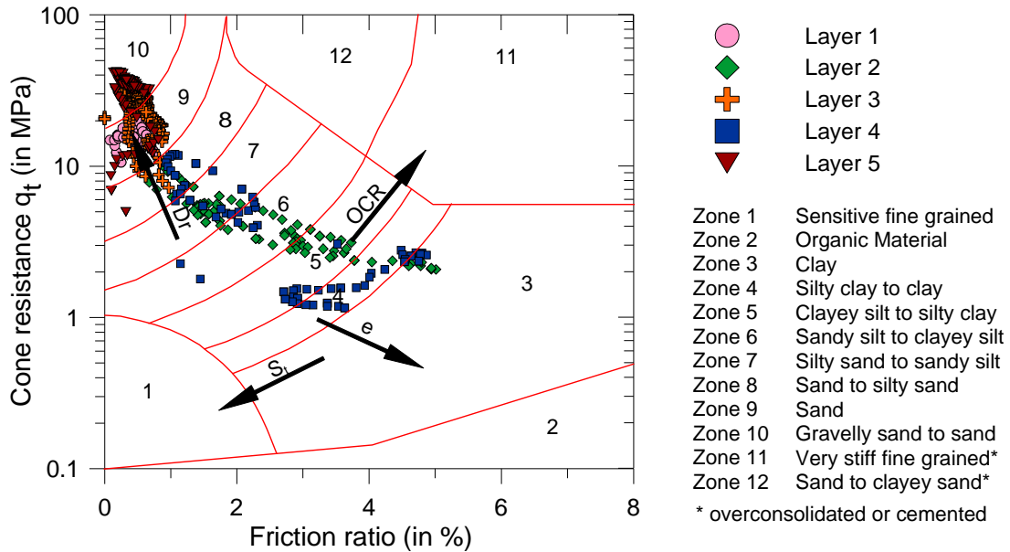
Figure 2: Soil Interpretation after Robertson et al. (1986).
