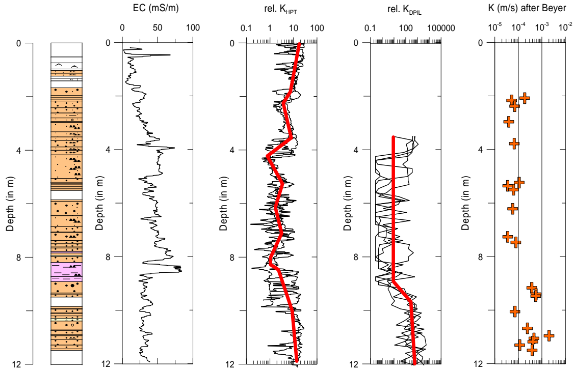
Figure 3: Comparison of the lithological profile; HPT and DPIL logs taken along a 150 m long profile, and preliminary results of calculated K -values after Beyer (1964) from grain size analyses.
