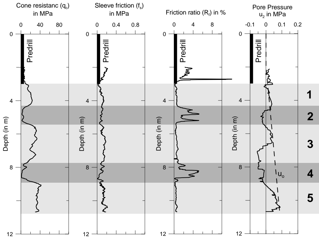
Figure 1: CPTU data showing q_c , f_s , R_f and u_2 and the layering based on the R_f .
